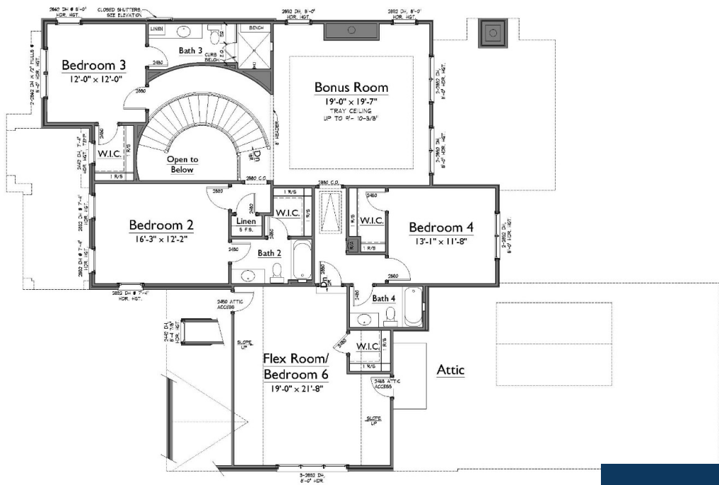
1 UPPER LEVEL FLOOR PLAN 1/8" = 1'-0"
